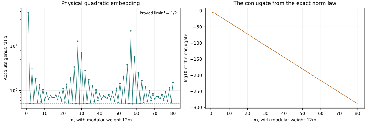
Figure 7.1: Numerical illustrations of the proved genus-ratio behavior at D = -15 . The physical embedding has large oscillations; its quadratic conjugate is computed from the exact norm law. Finite lattice sums supply the plotted values and explicit analytic tail budgets. The cluster theorem, not these finitely many points, proves the full interval of limit points.
