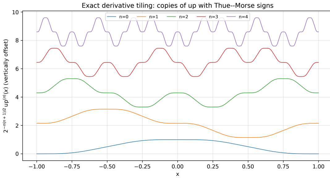
Figure 2: Normalized derivatives 2^{-T_n} up^{(n)} , vertically offset. Each row is a concatenation of copies of the original bump; their signs are the length- 2^n Thue–Morse block.
