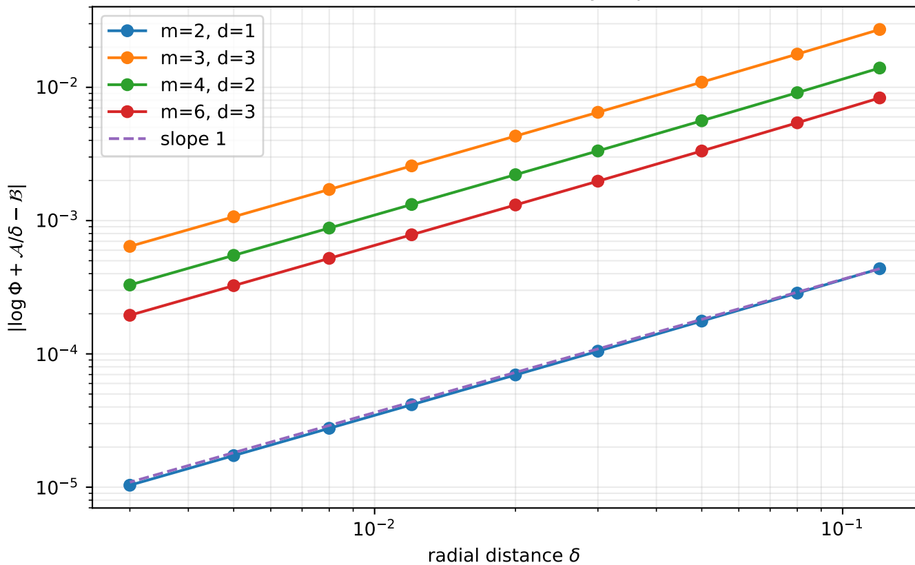
Two-term radial root-of-unity expansion
