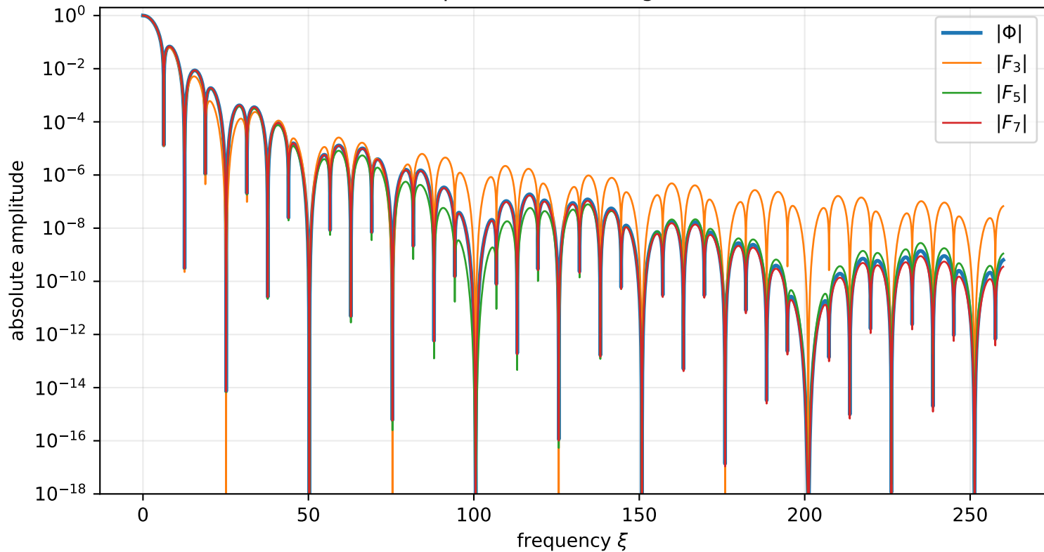
The finite products retain algebraic far tails
