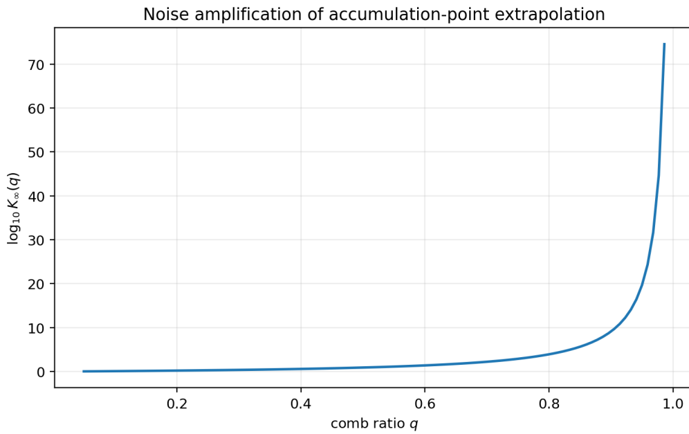
Figure 5: The infinite-order total variation K_{\infty}(q) = (-q; q)_{\infty} / (q; q)_{\infty} . The vertical axis is logarithmic in base 10. Stability is excellent for small and moderate q but deteriorates nonperturbatively as q \uparrow 1 .
