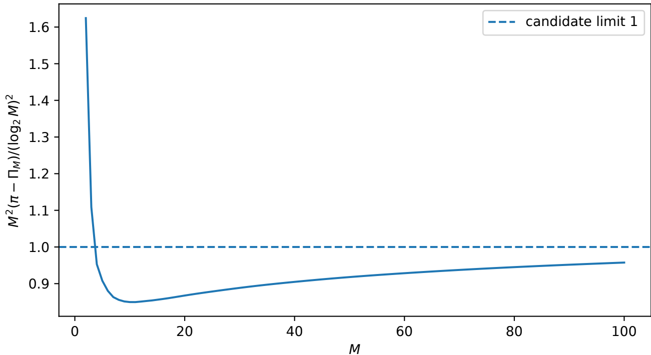
Scaled error of the rational Jacobi product for pi
