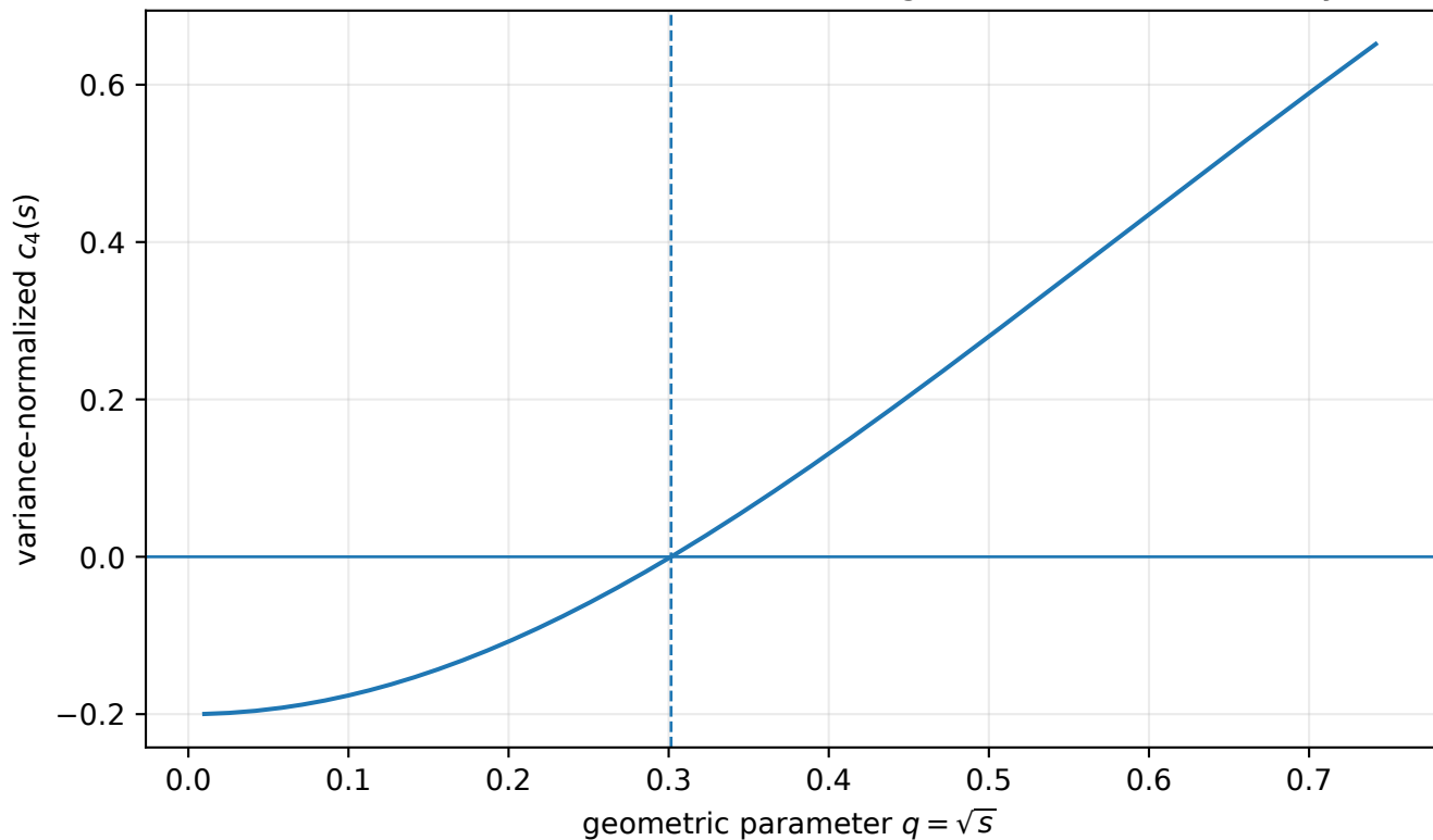
First free-cumulant obstruction in the geometric-uniform family
