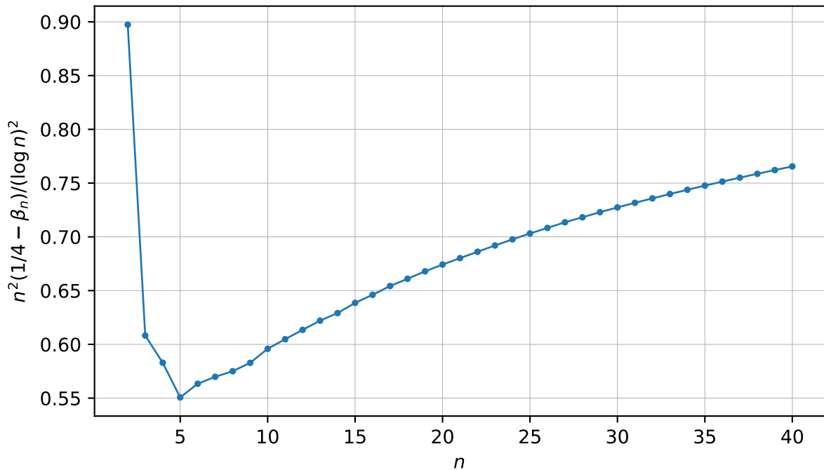
A diagnostic for the unresolved Jacobi-parameter rate
