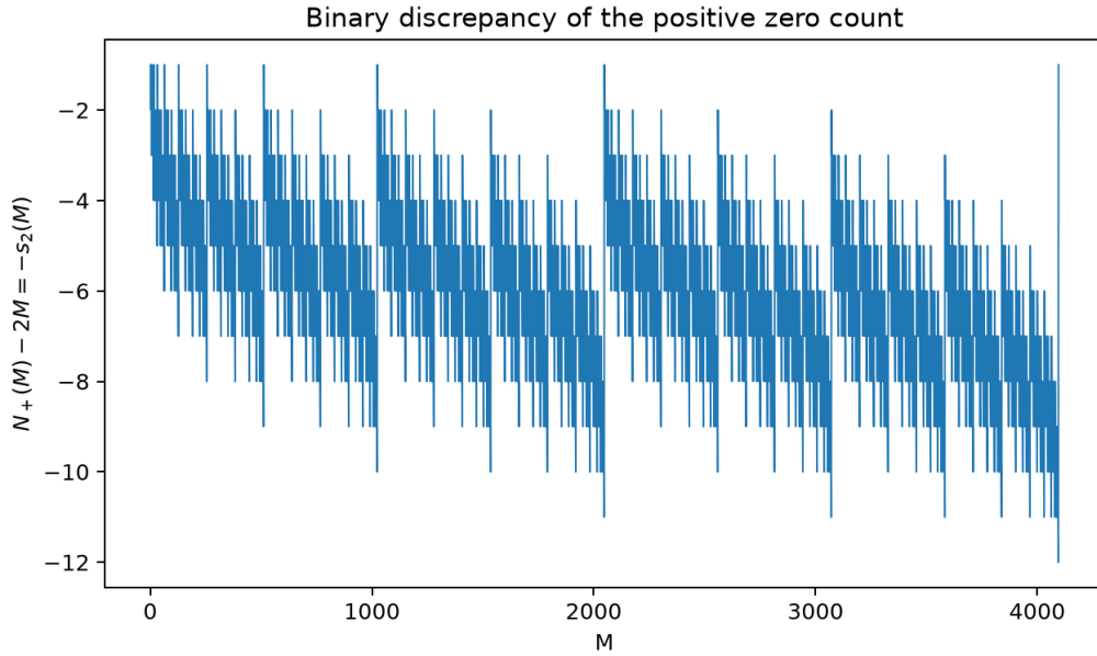
Figure 1: The exact discrepancy Z_+(M) - 2M = -\text{wt}_2(M) . The nested sawtooth pattern is not numerical noise: every plotted value is an integer identity.
