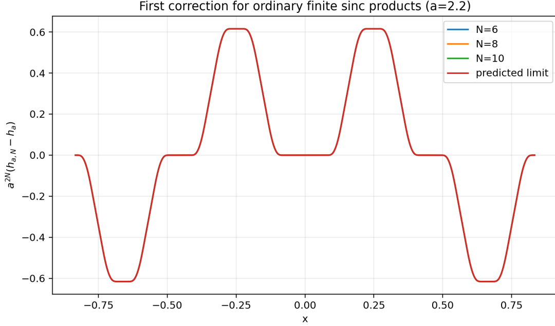
Figure 21: For a = 2.2 , the scaled errors a^{2N}(h_{a,N} - h_a) for N = 6, 8, 10 are visually indistinguishable from -h_a''/[6(a^2 - 1)] . The computation uses FFT inversion of the explicit products, not random sampling.
