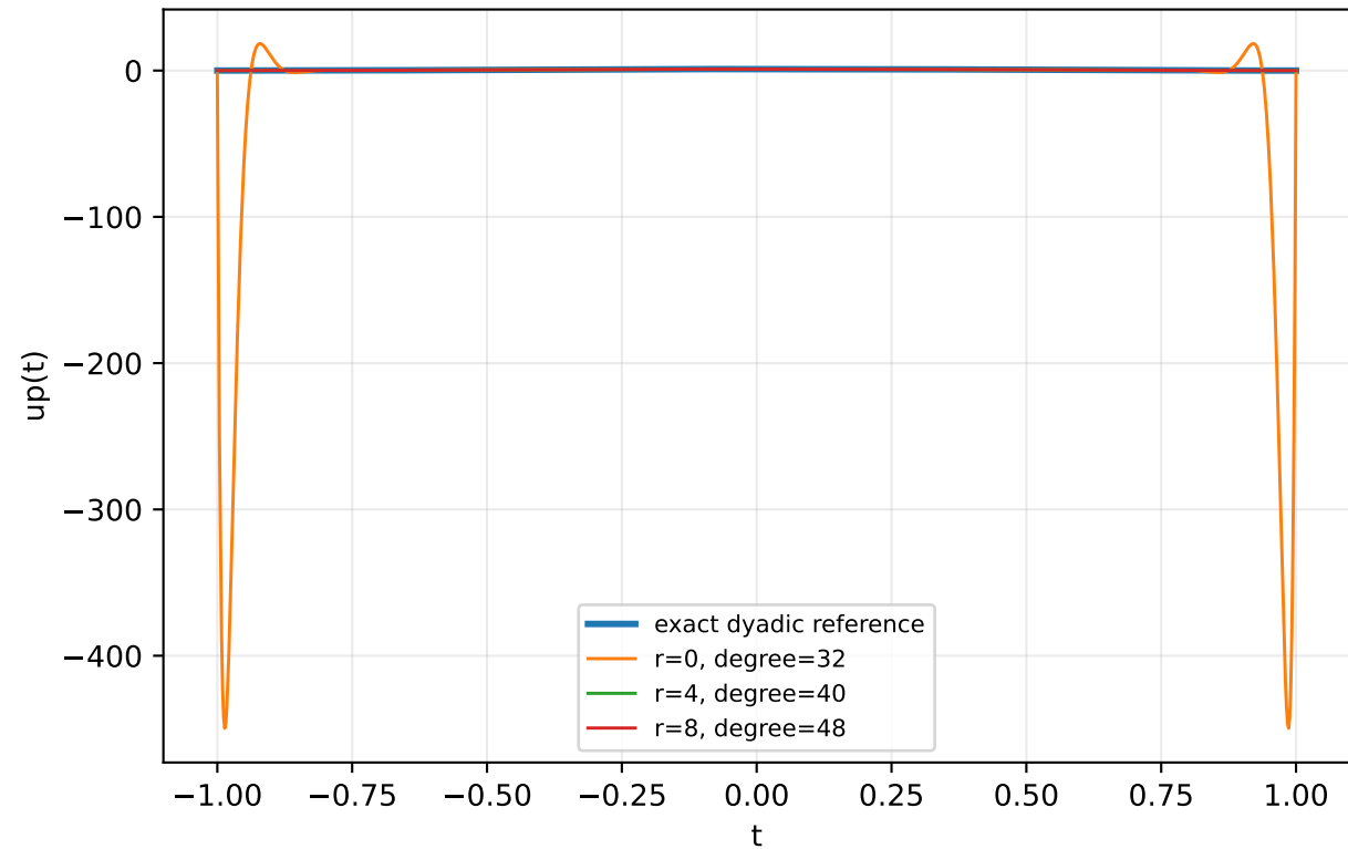
Endpoint-flat global interpolation: Rvachev up, N=32
