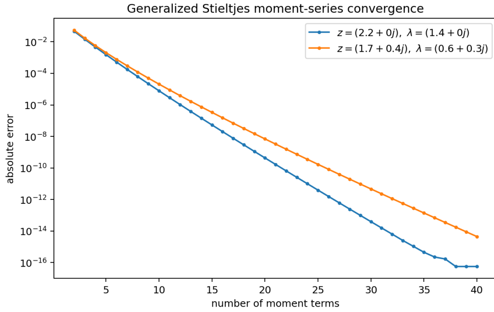
Figure 12: Convergence of the exact-moment expansion (1522) at two real/complex parameter pairs.
