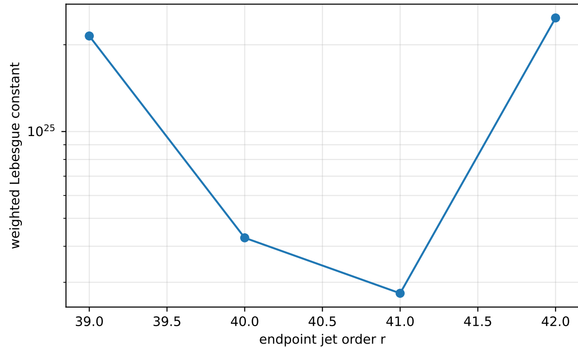
Endpoint-jet operator conditioning, N=256
