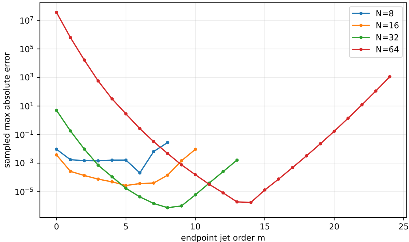
Fabius interpolation: a narrow finite-N stabilization window
