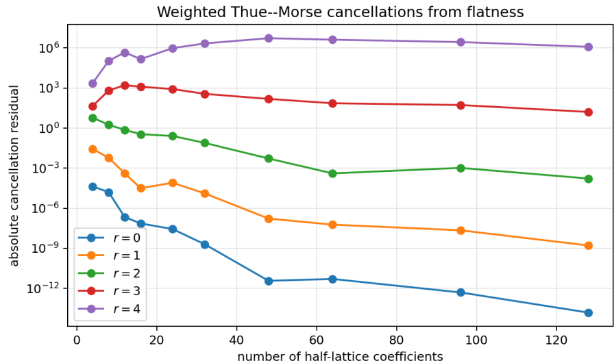
Figure 17: Truncation residuals in the spectral Prouhet identities (960). Higher powers initially amplify the tail before the super-polynomial Fourier decay dominates.
