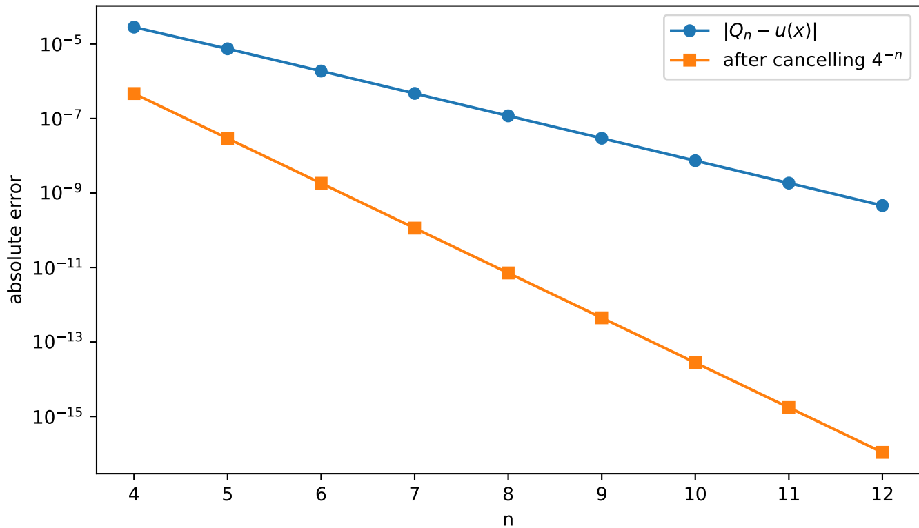
Geometric mode cancellation at x = 15/16
