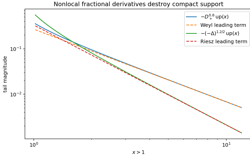
Figure 14: Weyl and Riesz fractional derivatives outside the support of u_p . Dashed curves are their leading x^{-1-\alpha} terms. The agreement illustrates how noninteger differentiation creates exact algebraic tails.
