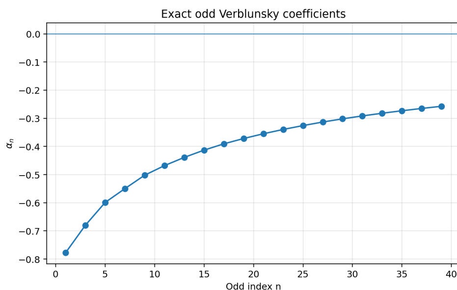
Figure 22: The first twenty exact odd Verblunsky coefficients. All even coefficients vanish. The displayed odd values are negative and increase toward zero, motivating Theorem 10.1; Rakhmanov’s theorem proves convergence to zero but not the observed sign and monotonicity.
