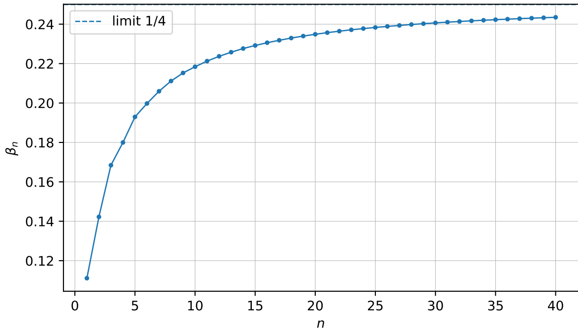
Jacobi coefficients of the Rvachev up-law
