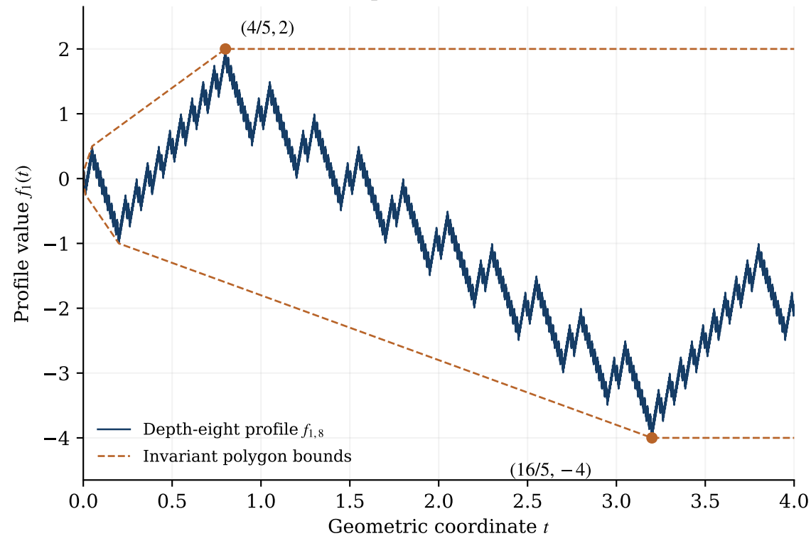
(a) Self-affine profile and exact contacts
