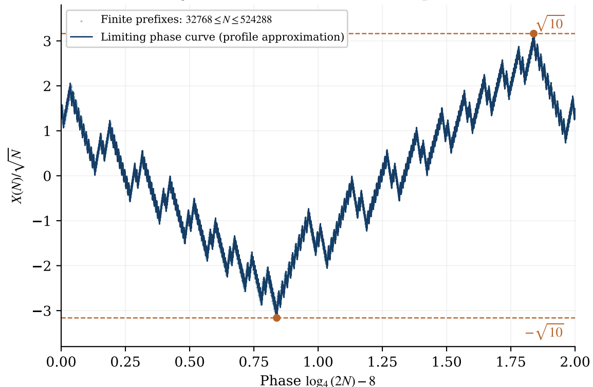
(b) Physical normalization and the phase law
