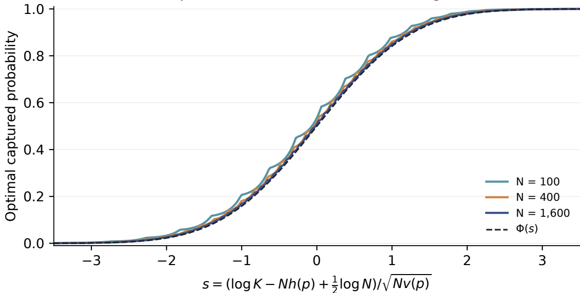
Fixed bias p = 0.1 : the normal candidate-budget transition
