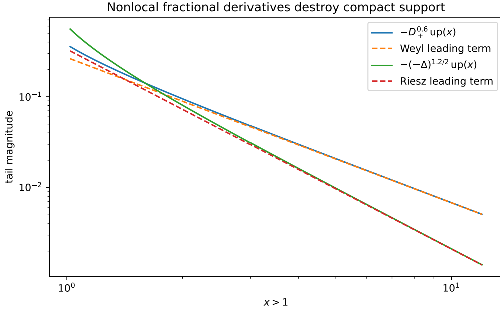
Figure 14: Weyl and Riesz fractional derivatives outside the support of up . Dashed curves are their leading x^{-1-\alpha} terms. The agreement illustrates how noninteger differentiation creates exact algebraic tails.
