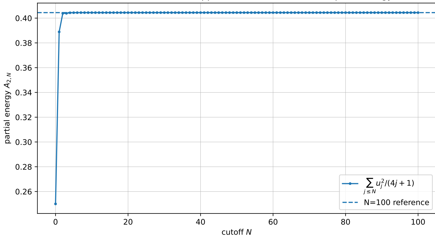
Monotone exact-rational approximation to the Fabius square energy
