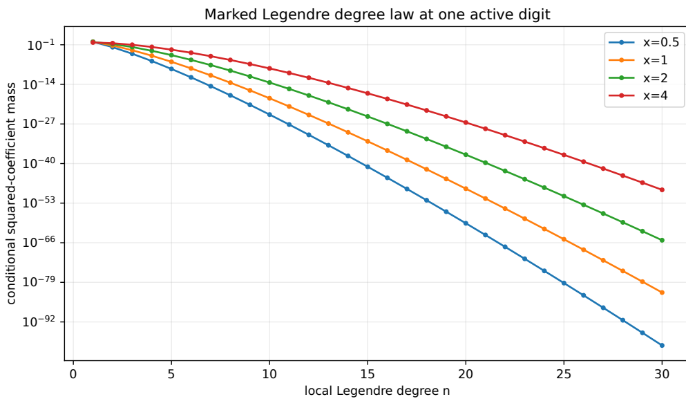
Figure 2: The local degree mark in (50). Larger local field x activates higher Legendre degrees, while the far dyadic tail remains almost entirely degree one when it activates.
