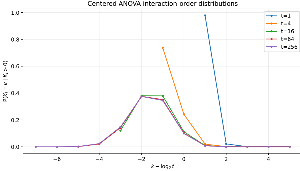
Figure 1: Exact Poisson–binomial order weights \mathbb{P}(K_t = k \mid K_t > 0) for several values of t . As t increases, the interaction order translates roughly by \log_2 t rather than widening on a central-limit scale.
