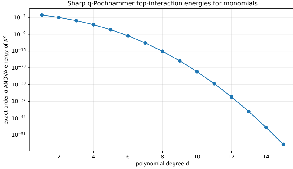
Figure 3: The exact highest-order interaction energy (72). The quadratic exponent in the dyadic factor forces superexponential decay even after multiplication by (d!)^2 .
