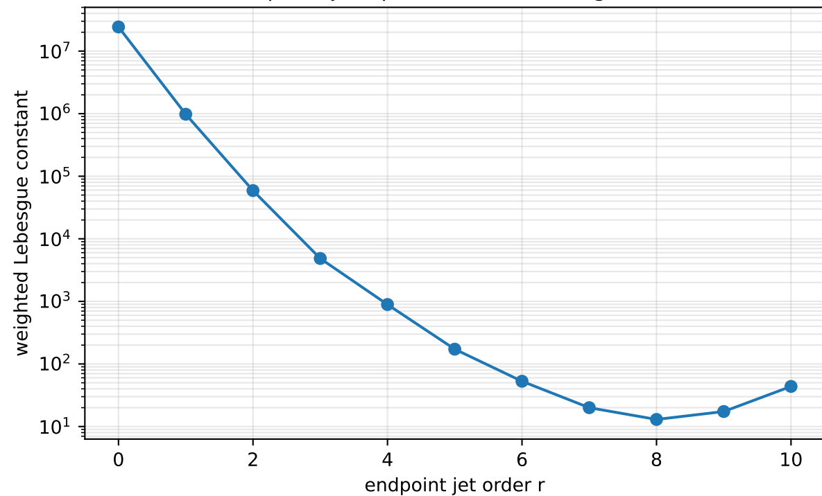
Endpoint-jet operator conditioning, N=32
