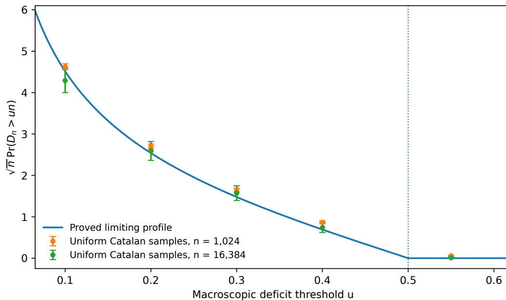
Figure 7: Manuscript 10: the proved macroscopic tail profile \Psi and uniform Catalan sampling illustrations at n = 1,024 and 16,384 , from the shipped simulation data of table 16. Error bars show two estimated Monte Carlo standard errors; they do not bound finite-size bias and are not rigorous confidence certificates. In particular, positive finite-size tails beyond u = 1/2 are compatible with the limiting zero there.
