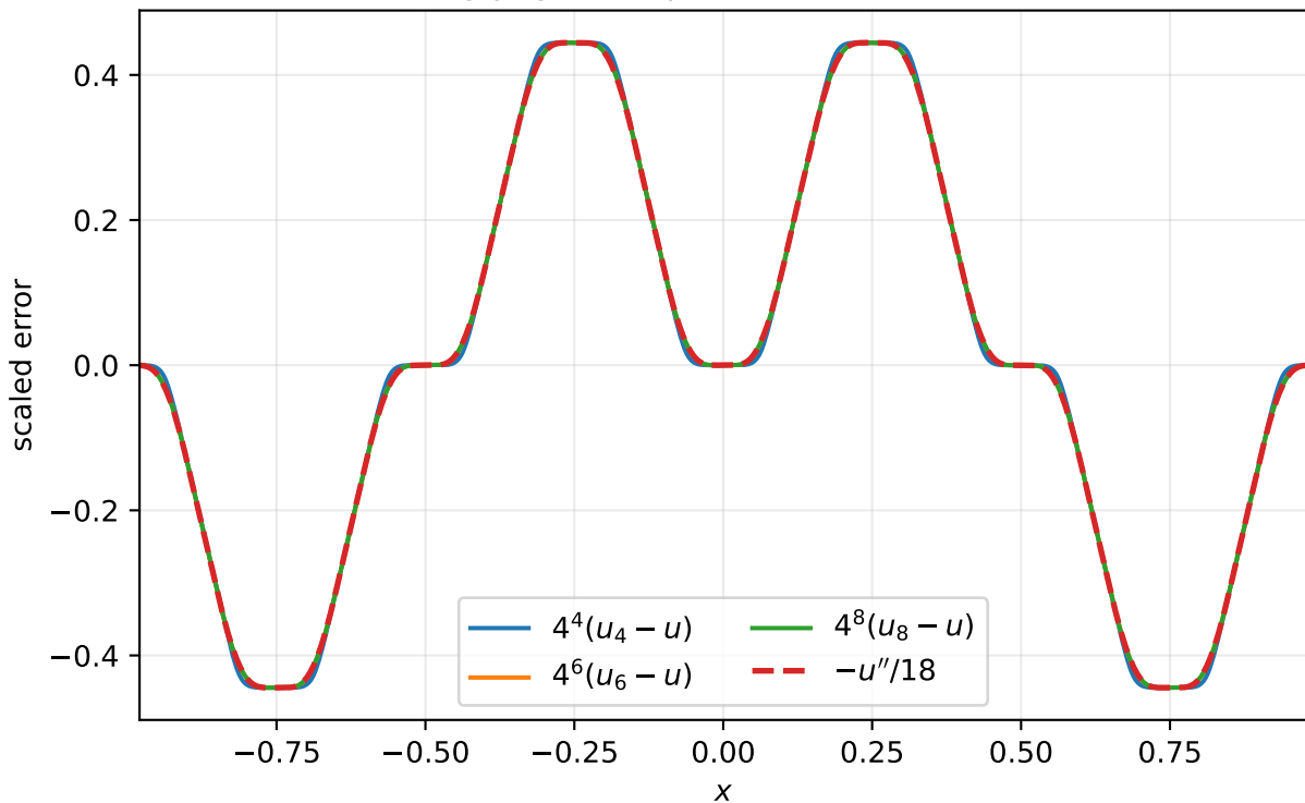
Leading physical-space deconvolution error
