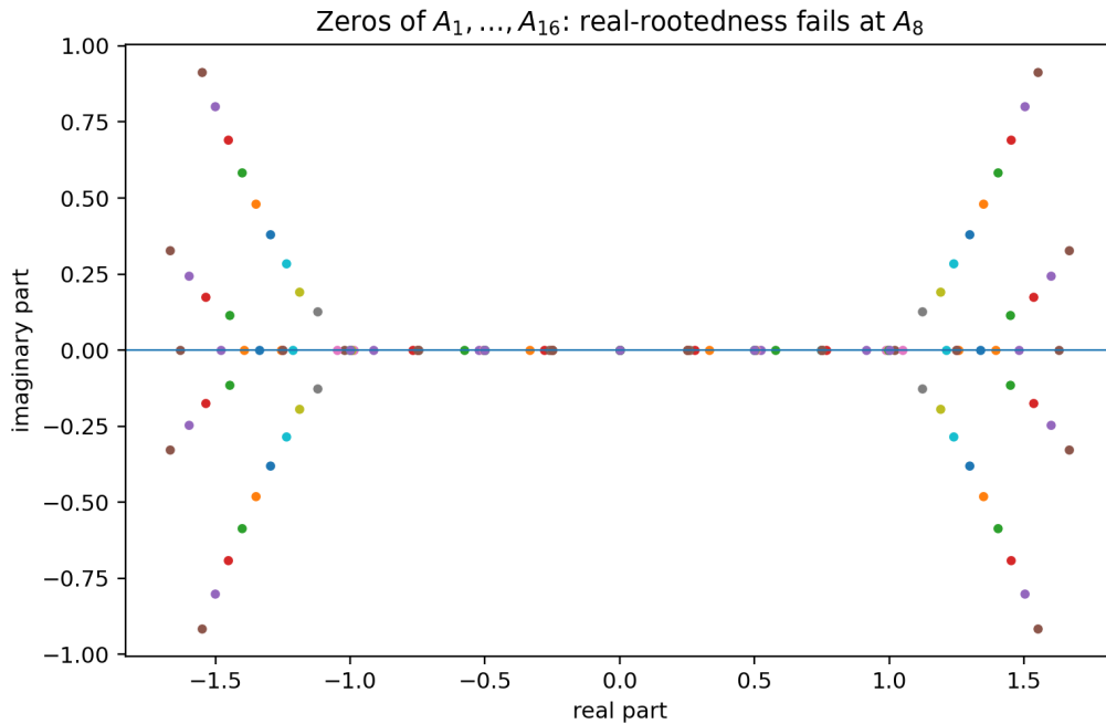
Figure 3: Numerical locations of the zeros of \mathcal{A}_1, \dots, \mathcal{A}_{16} . The exact Sturm result certifies the first departure from the real axis at degree eight; the later pattern is exploratory.
