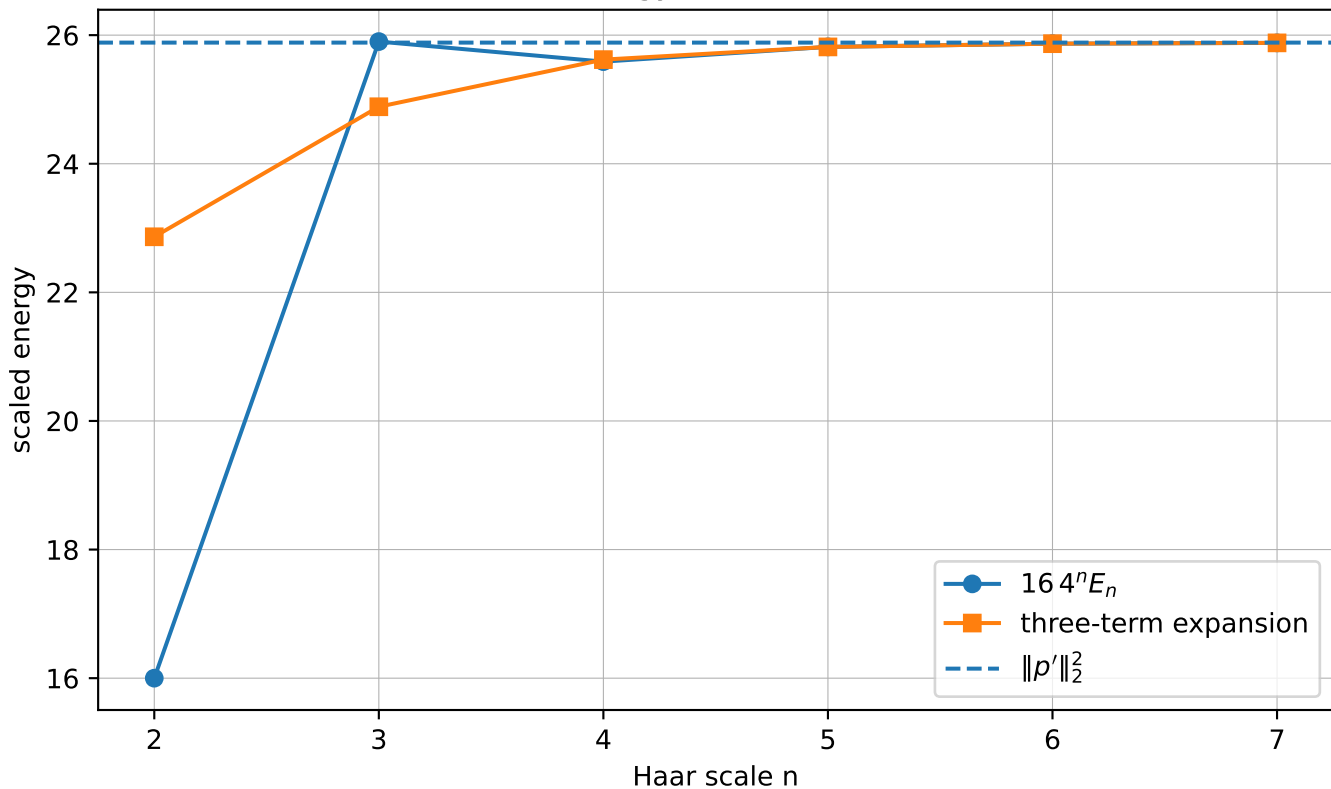
Haar detail energy and its continuum limit
