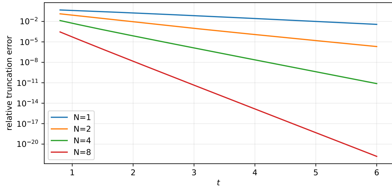
Exact 2-adic exponential tail B(t)
