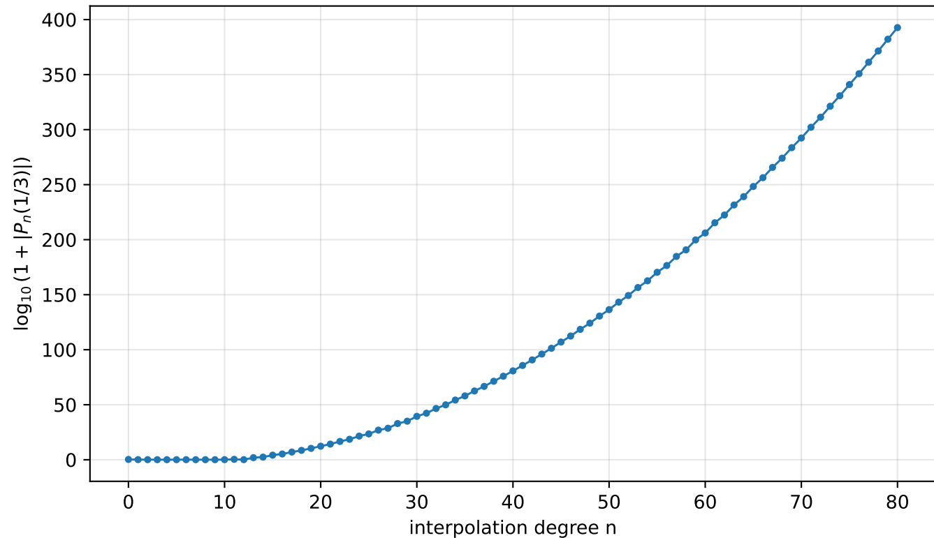
Fabius Newton interpolants diverge away from the geometric comb
