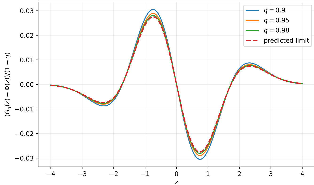
First non-Gaussian correction
