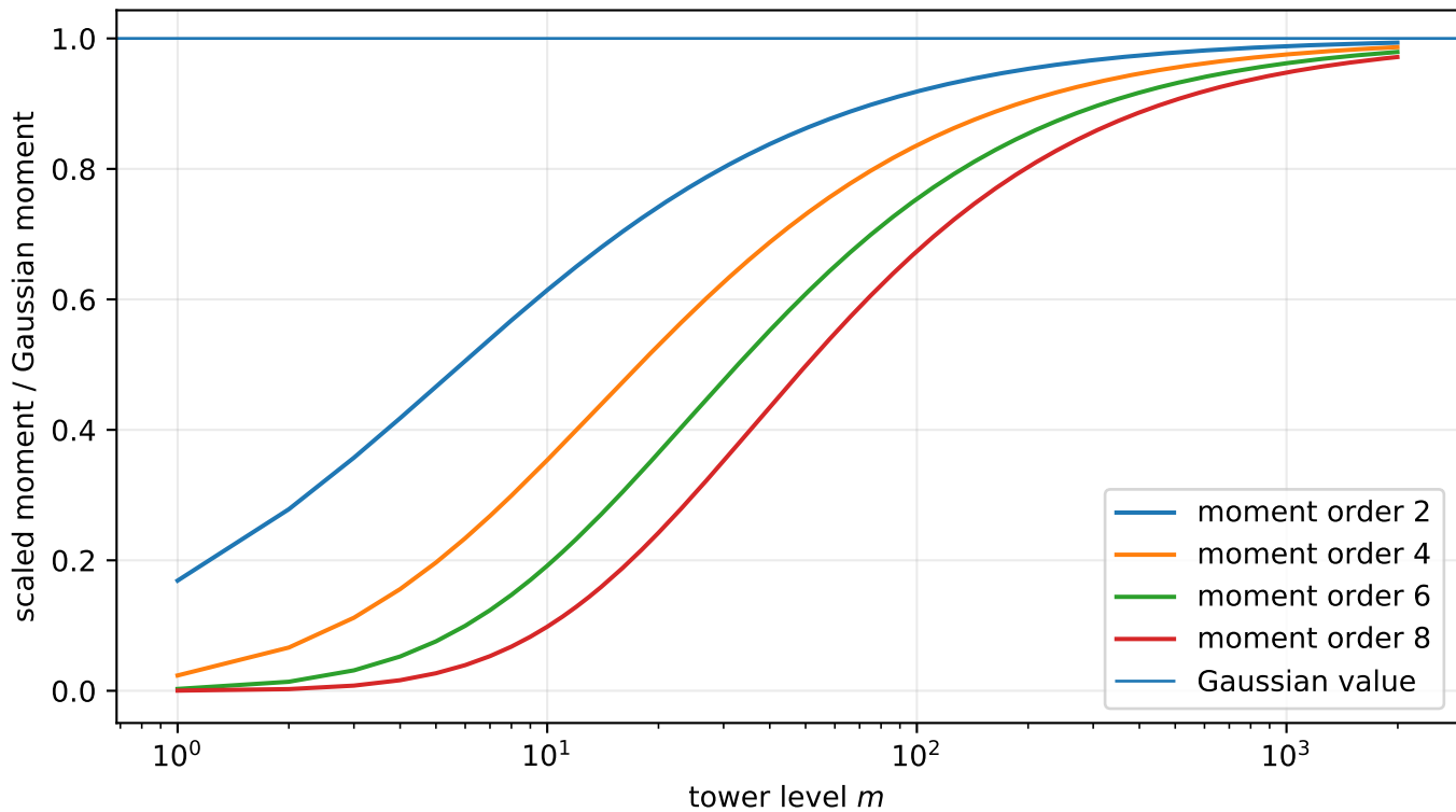
Gaussianization of \sqrt{2m} \gamma^{[m]}
