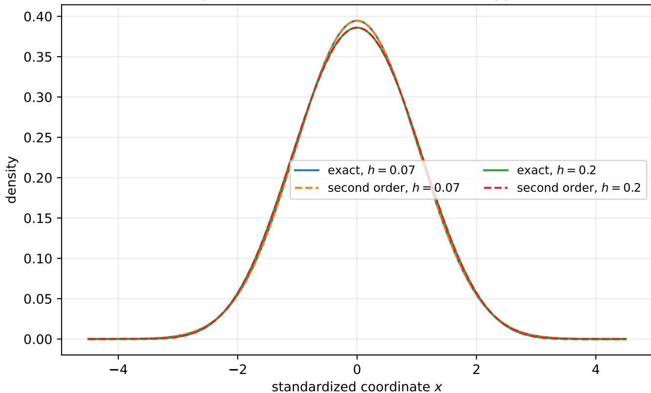
Exact sinc-product densities and second-order approximation
