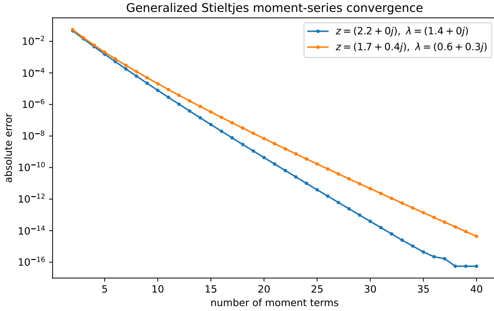
Figure 12: Convergence of the exact-moment expansion (1504) at two real/complex parameter pairs.
