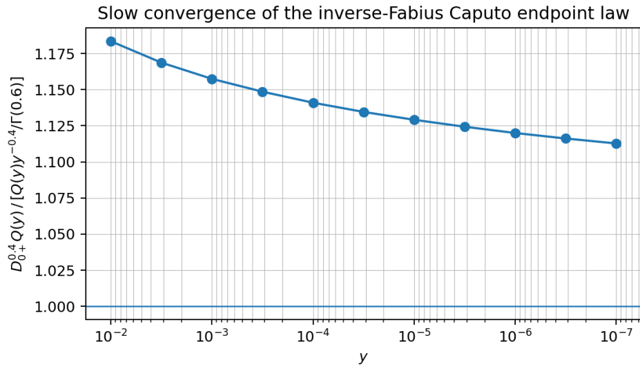
Figure 9: The ratio in equation (1124) for r = 1 and \beta = 0.4 . The theorem predicts convergence to 1; the slow drift exposes the scale of the first Lambert-type correction.
