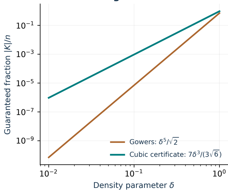
Common-neighborhood core size
