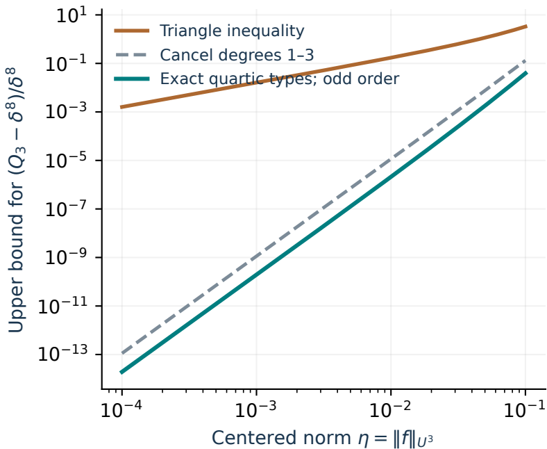
Cube-count error: d = 3, \delta = 1/2
