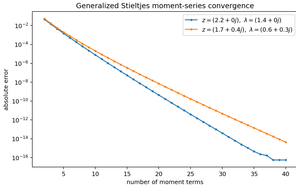
Figure 12: Convergence of the exact-moment expansion (1507) at two real/complex parameter pairs.
