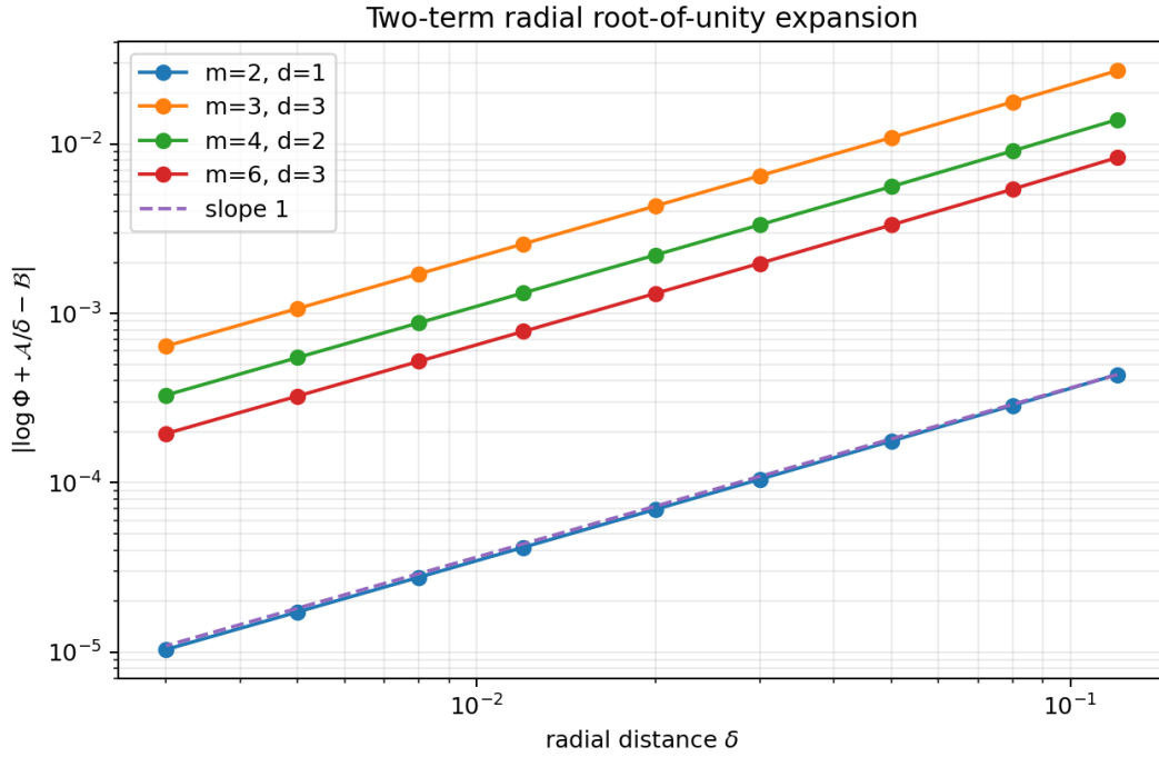
Figure 42: For z = 0.8 , the residual |\log \Phi + \mathcal{A}/\delta - \mathcal{B}| is asymptotically linear in \delta at four root orders. The fitted slopes over the five smallest radial distances are all between 1.0043 and 1.0045.
