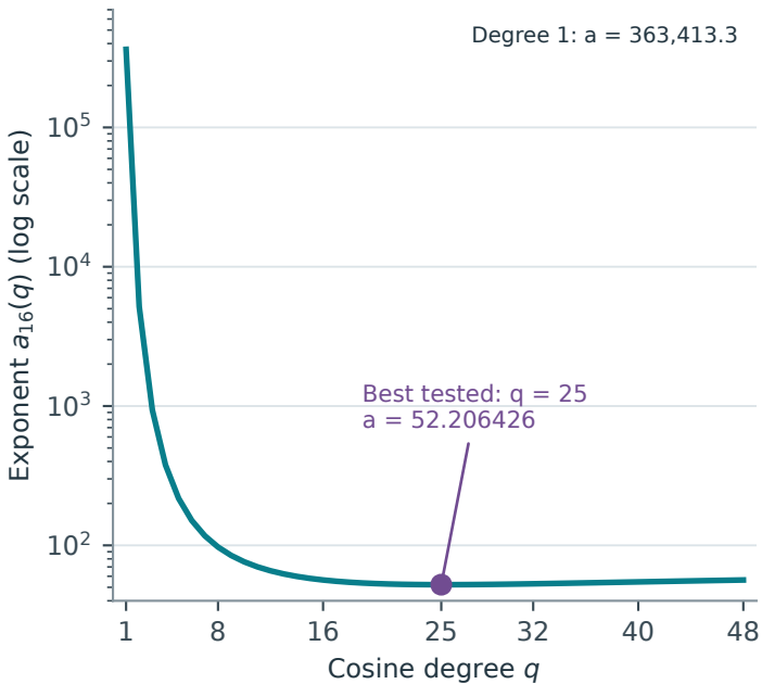
(a) Sixteen variables
