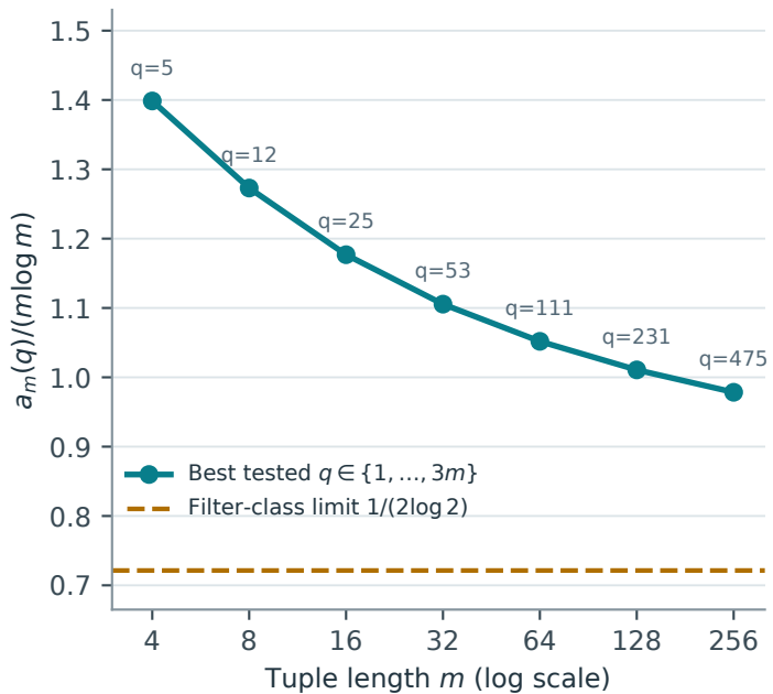
(b) Growth of the exponent
