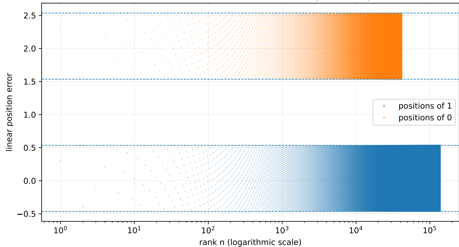
A284368: errors remain inside much sharper envelopes
