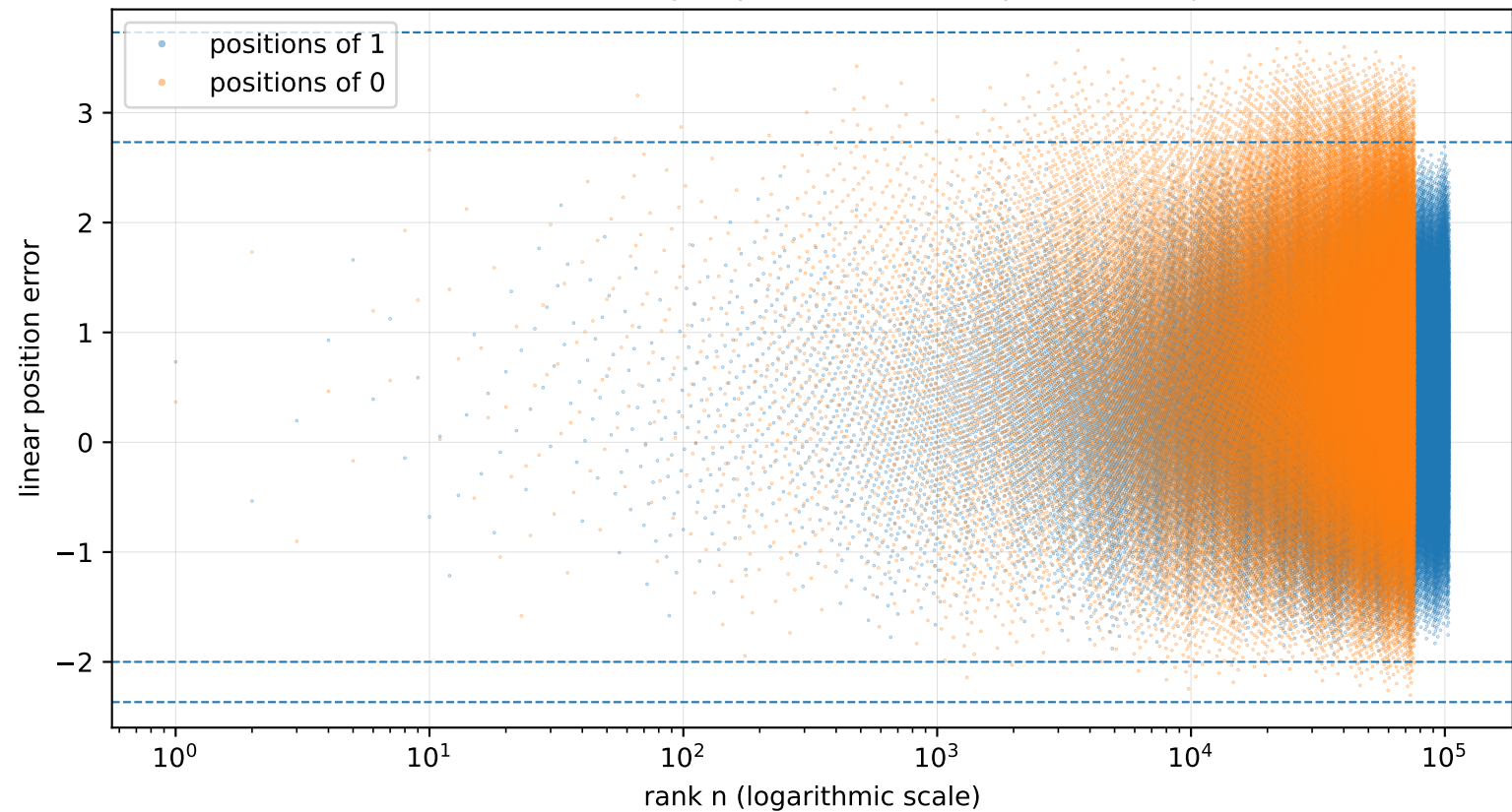
A284369: exact envelopes prove both OEIS position conjectures
