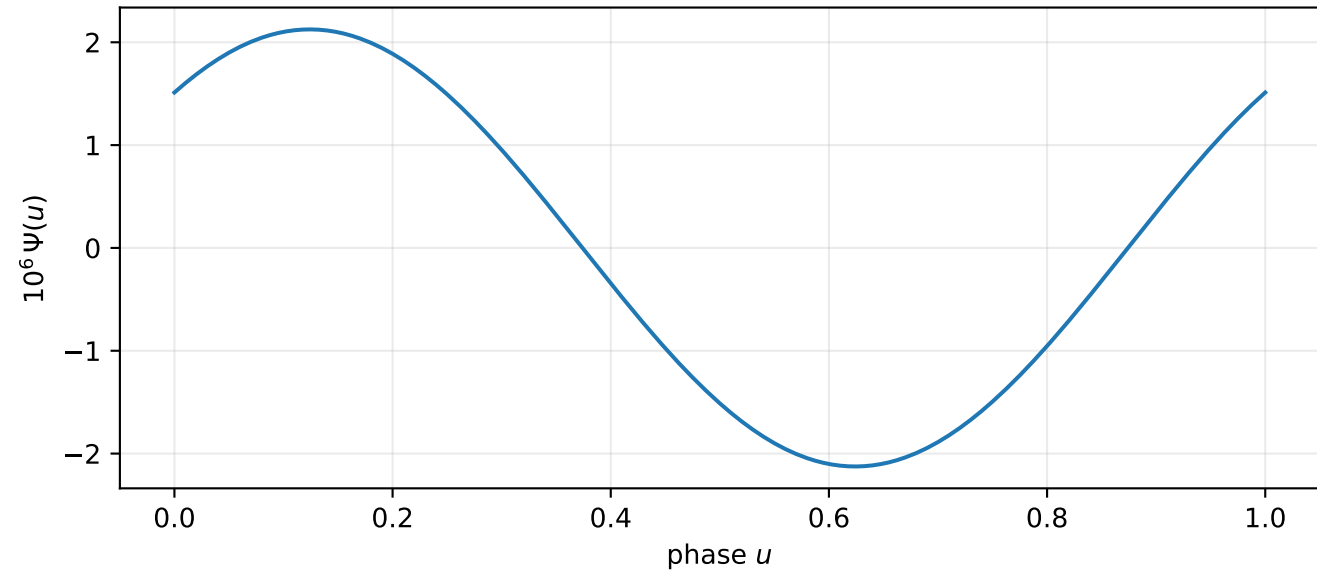
Gamma--zeta periodic correction
