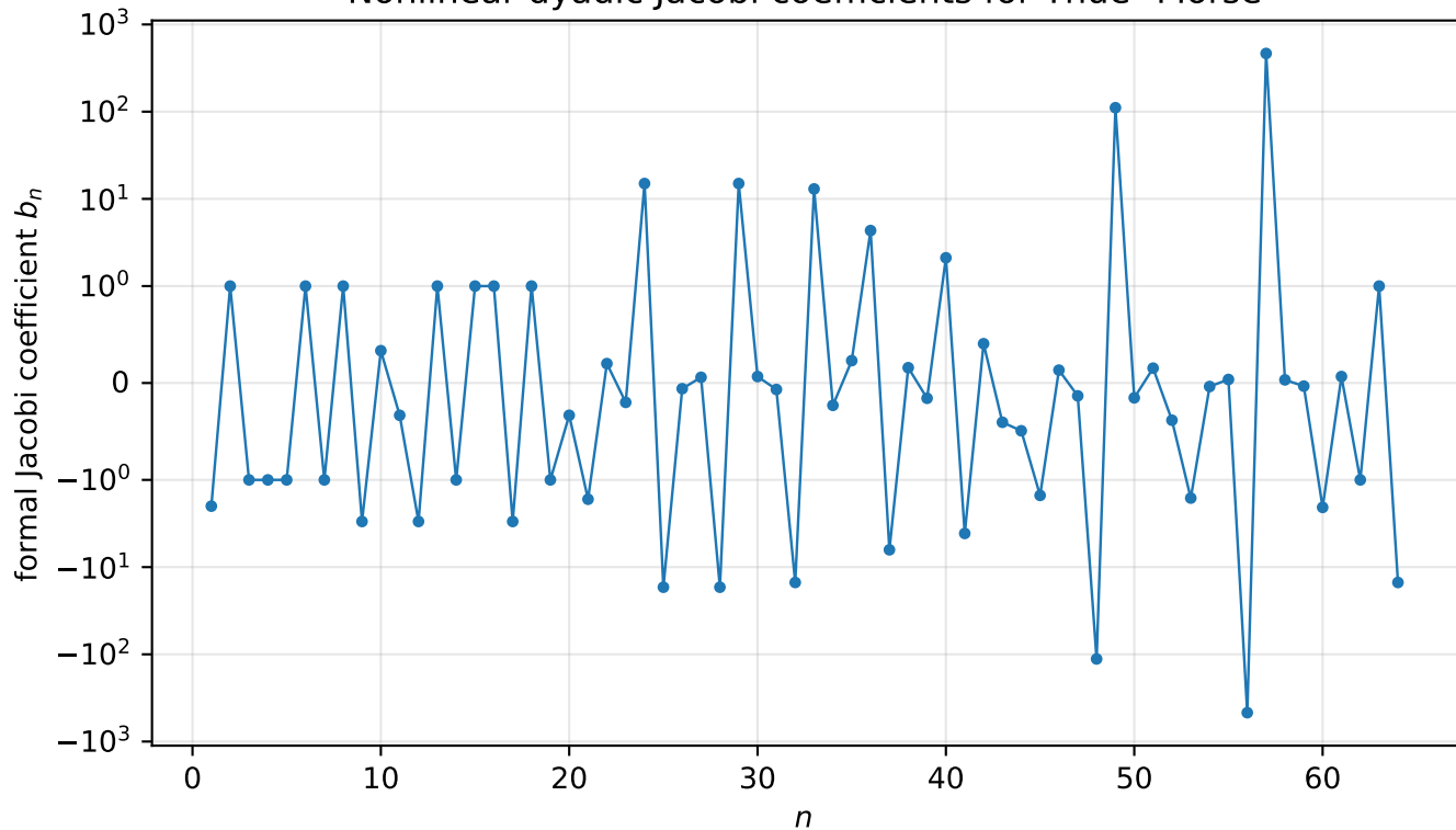
Nonlinear dyadic Jacobi coefficients for Thue--Morse
