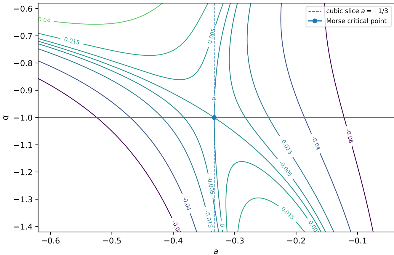
Level geometry of (a; q)_3 near (-1/3, -1)
