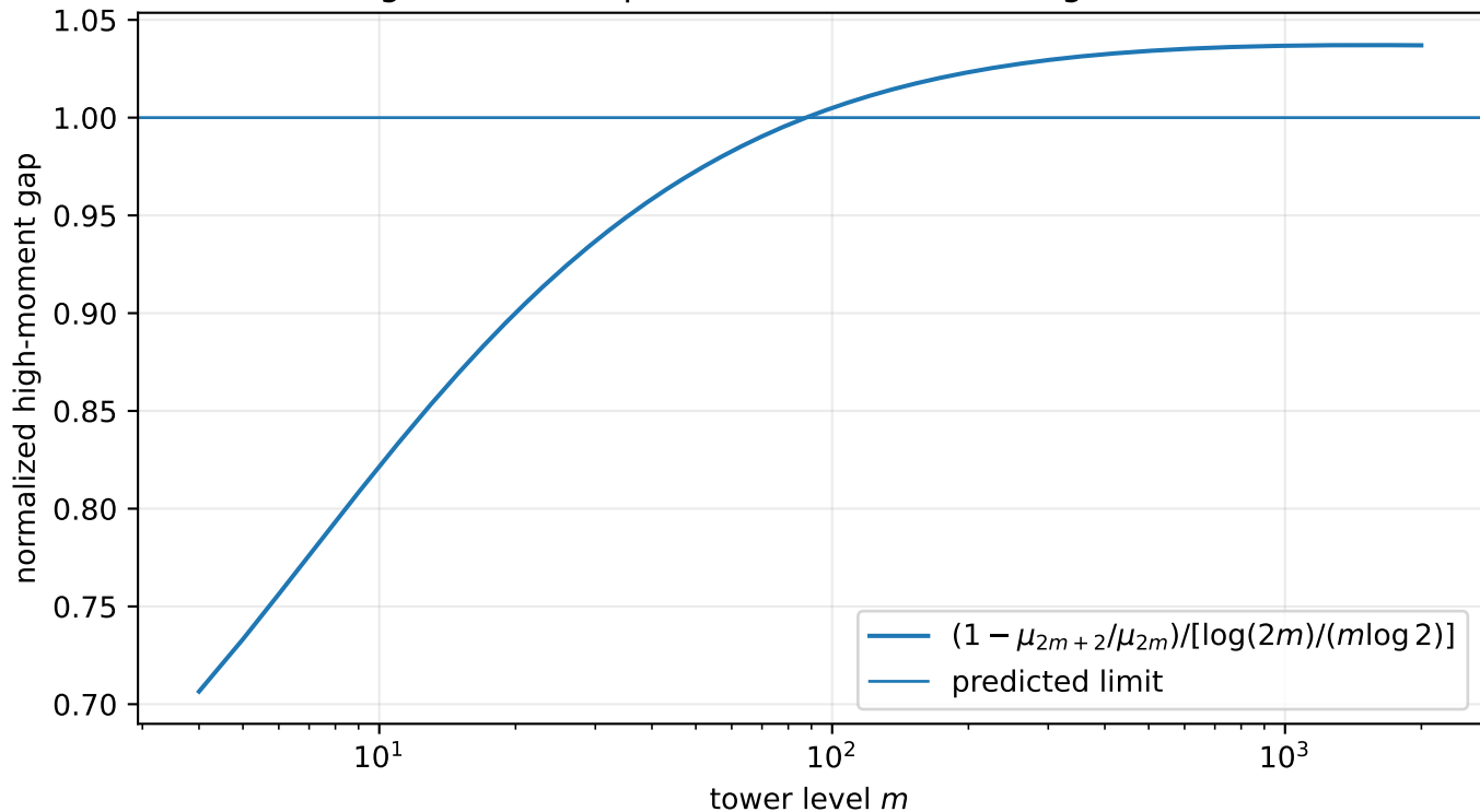
Logarithmic endpoint scale in Rvachev high moments
