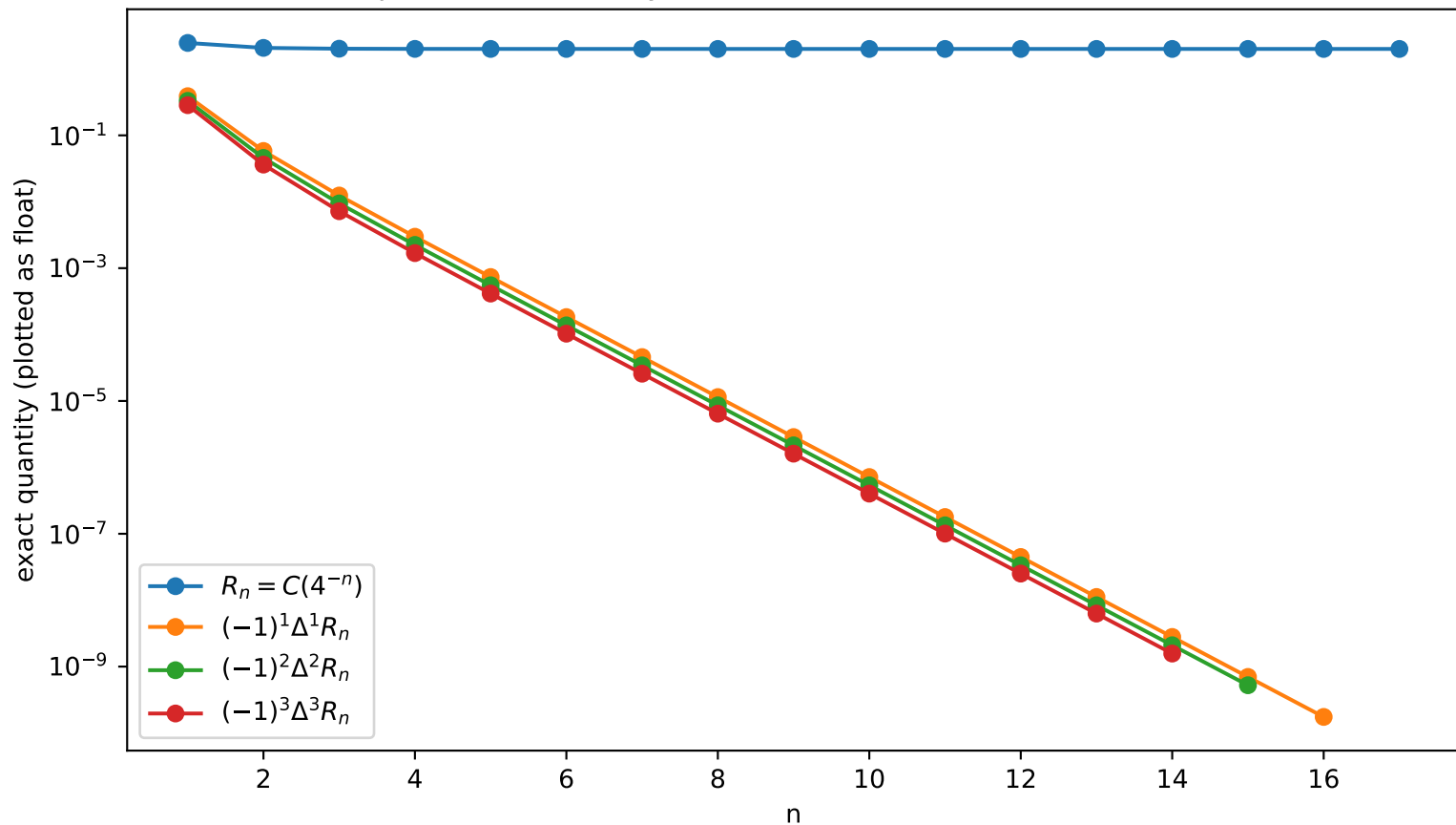
Complete monotonicity of the normalized even-cumulant ratios
