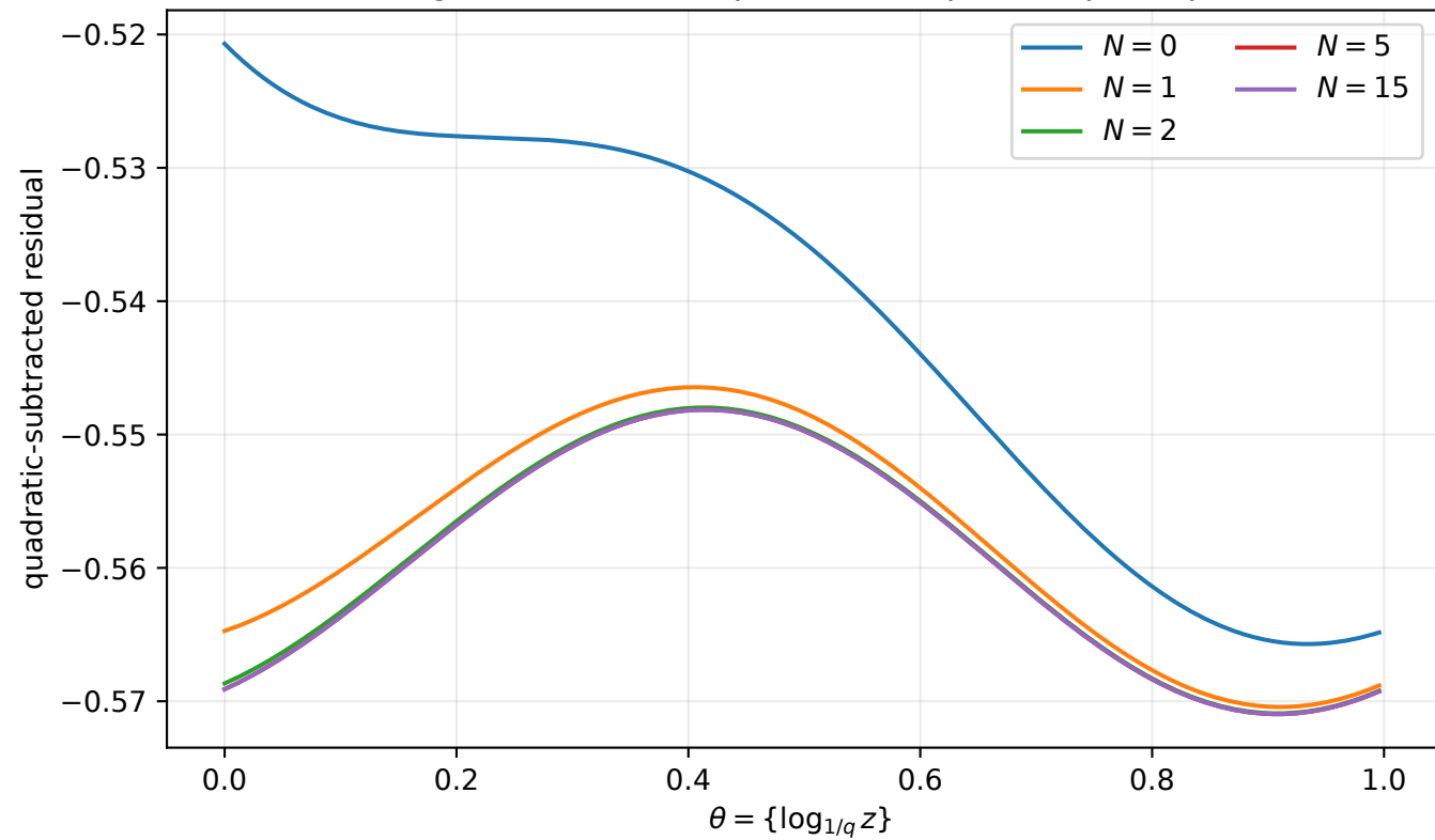
Convergence to the one-periodic endpoint Laplace profile
