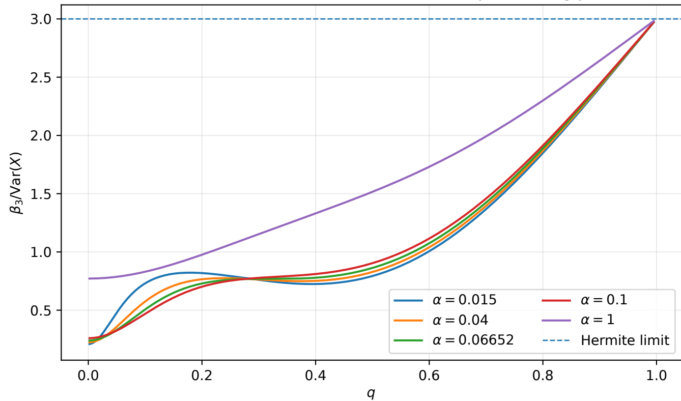
Third recurrence coefficient and the small- \alpha turning phase
