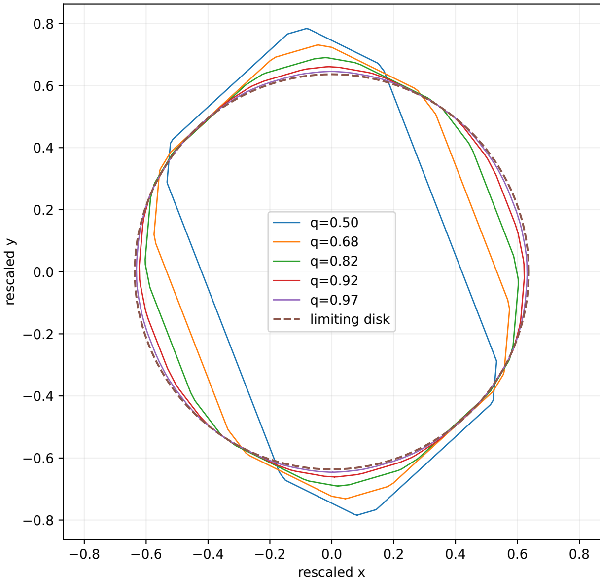
Abel rescaling of irrational rotating zonoids
