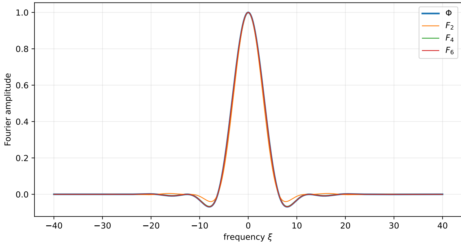
Finite repeated-integration spectra
